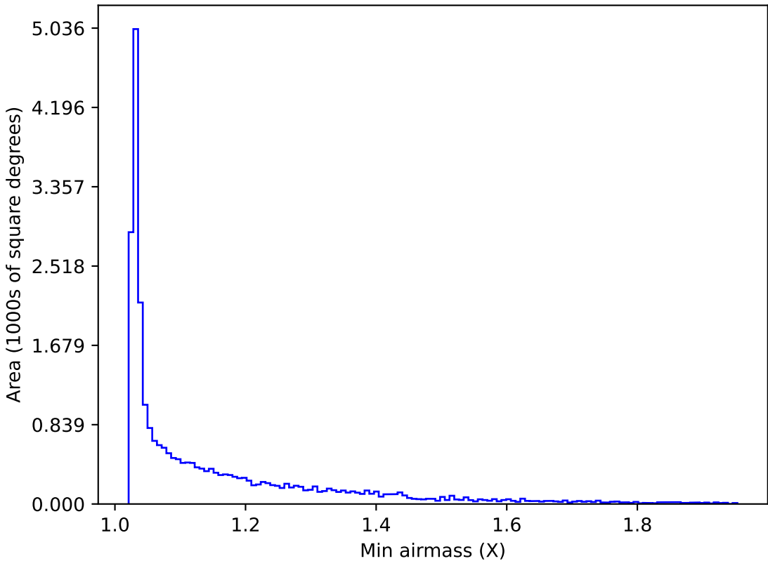
ddf_acor_sf10_lsf15_lsr50_v3.4_10yrs Yr 1 all bands: Min airmass
