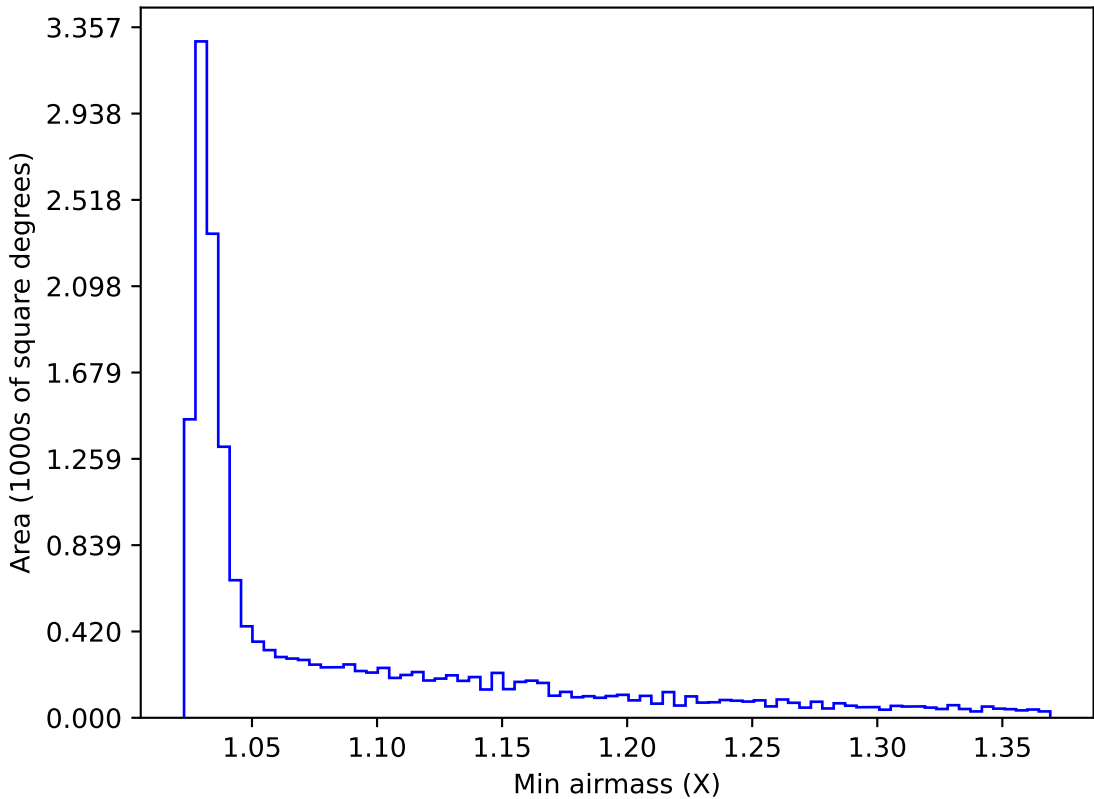
ddf_acor_sf10_lsf15_lsr50_v3.4_10yrs WFD y band: Min airmass
