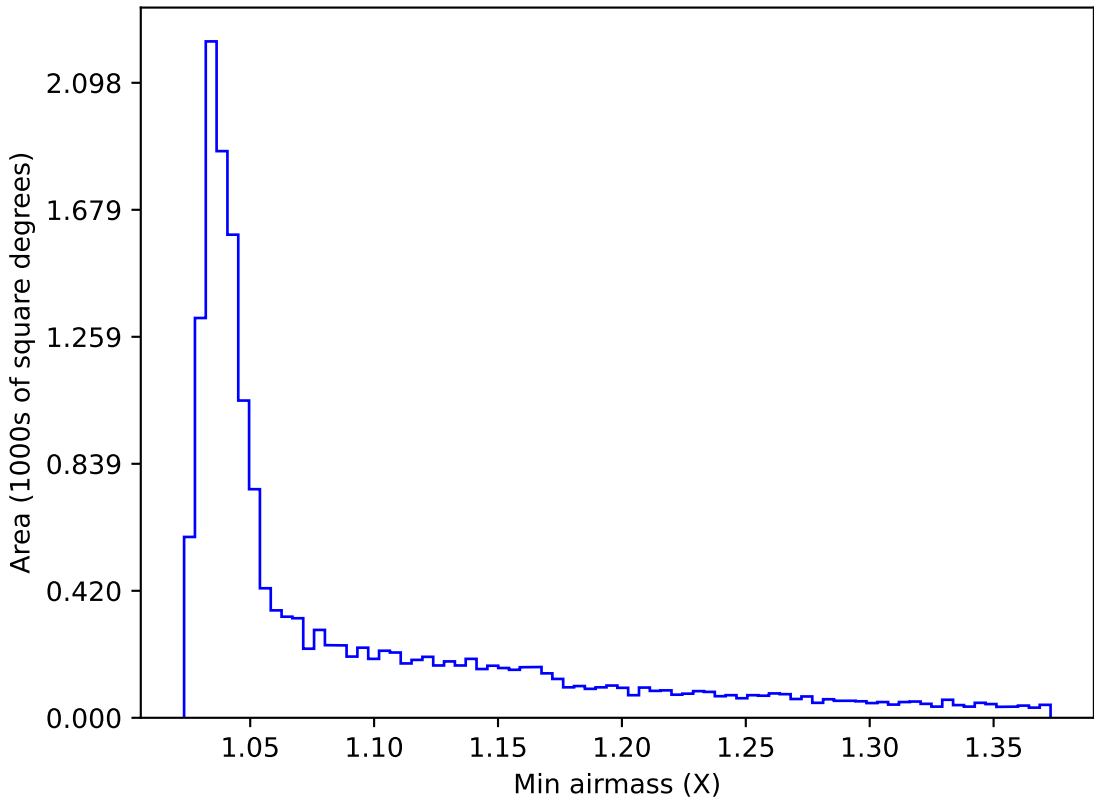
ddf_acor_sf10_lsf15_lsr50_v3.4_10yrs WFD u band: Min airmass
