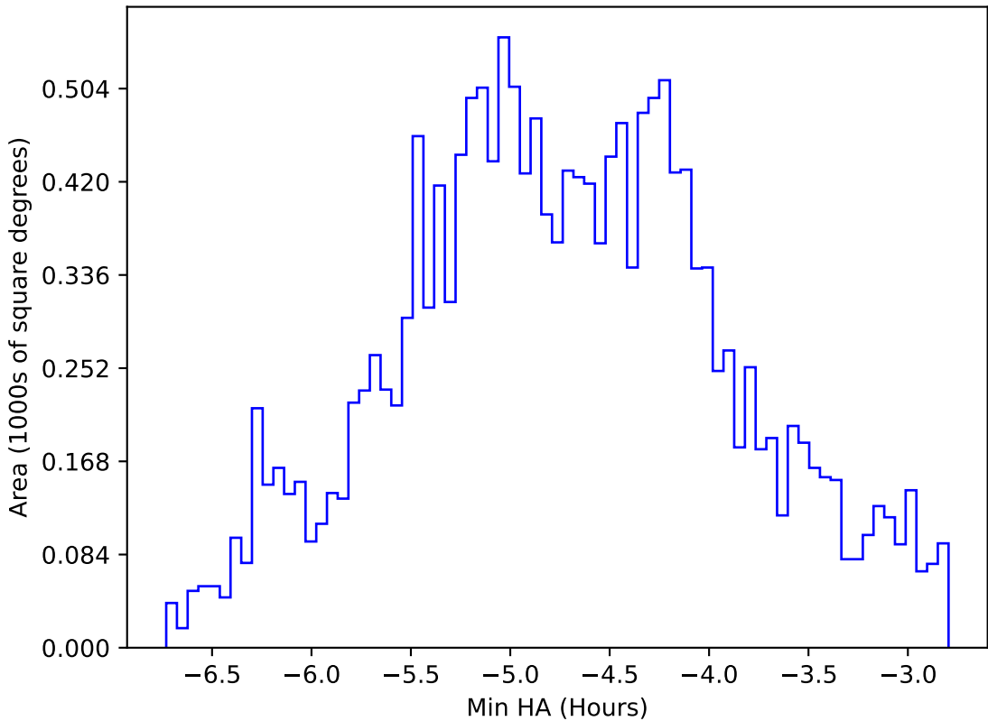
ddf_acor_sf10_ls15_lsr50_v3.4_10yrs WFD all bands: Min HA
