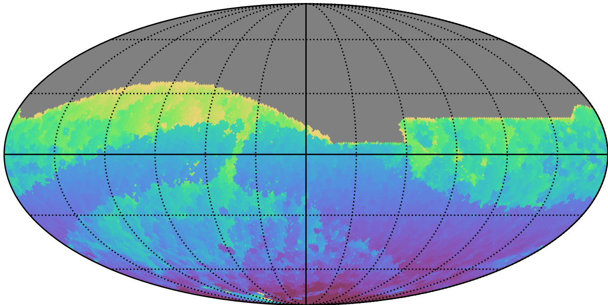
ddf_acor_sf10_lsf15_lsr50_v3.4_10yrs All sky r band: Min HA
