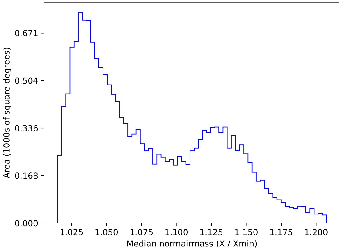
ddf_acor_sf10_lsf15_lsr50_v3.4_10yrs WFD g band: Median normairmass
