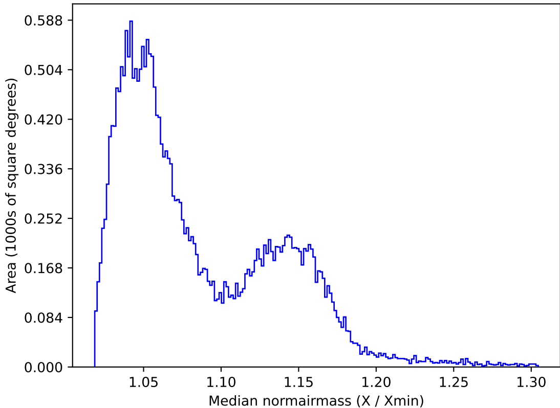
ddf_acor_sf10_ls15_lsr50_v3.4_10yrs All sky z band: Median normairmass
