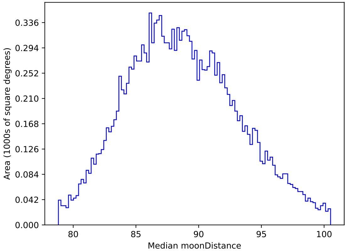
ddf_acor_sf10_lsf15_lsr50_v3.4_10yrs WFD all bands: Median moonDistance
