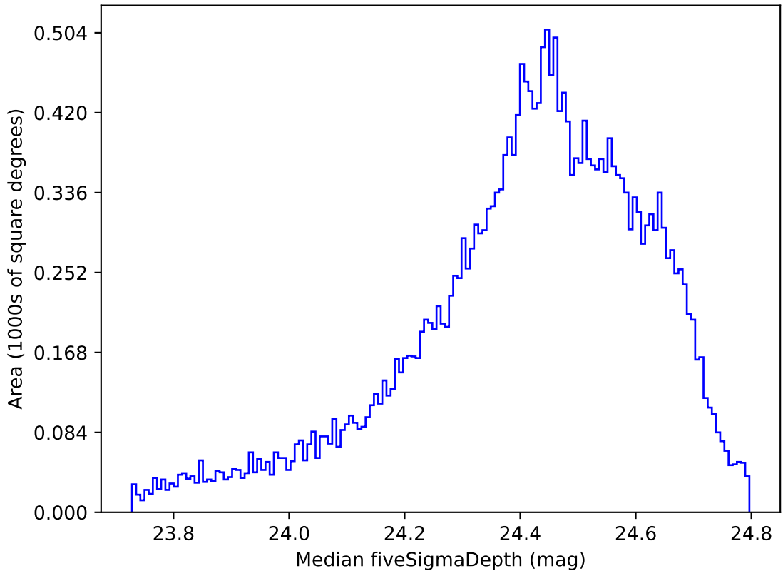
ddf_acor_sf10_lsf15_lsr50_v3.4_10yrs All sky g band: Median fiveSigmaDepth
