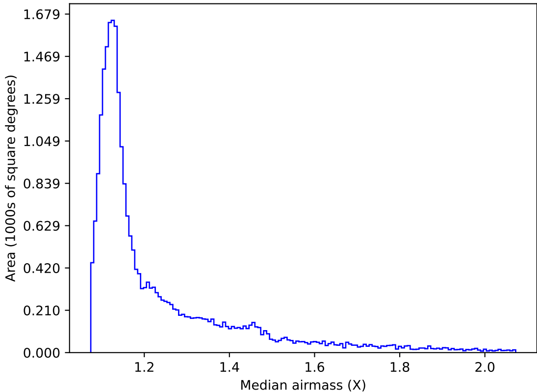
ddf_acor_sf10_lsf15_lsr50_v3.4_10yrs Yr 1 all bands: Median airmass
