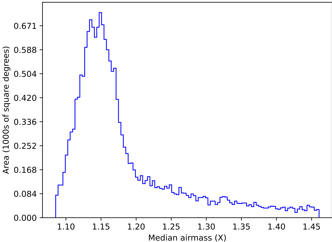
ddf_acor_sf10_lsf15_lsr50_v3.4_10yrs WFD z band: Median airmass
