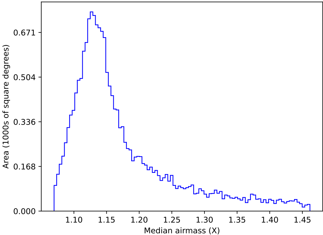
ddf_acor_sf10_ls15_lsr50_v3.4_10yrs WFD u band: Median airmass
