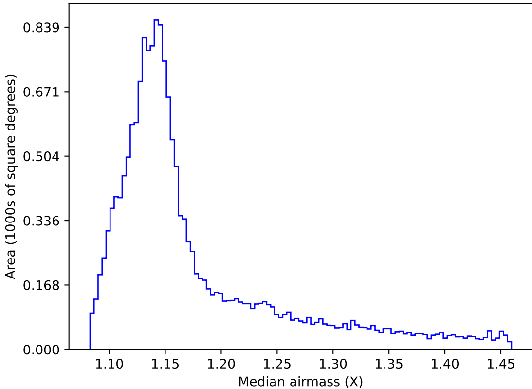
ddf_acor_sf10_lsf15_lsr50_v3.4_10yrs WFD all bands: Median airmass
