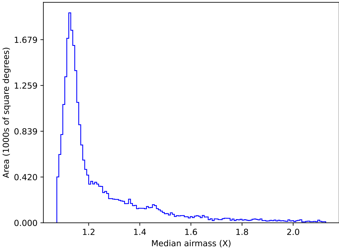
ddf_acor_sf10_lsf15_lsr50_v3.4_10yrs All sky r band: Median airmass
