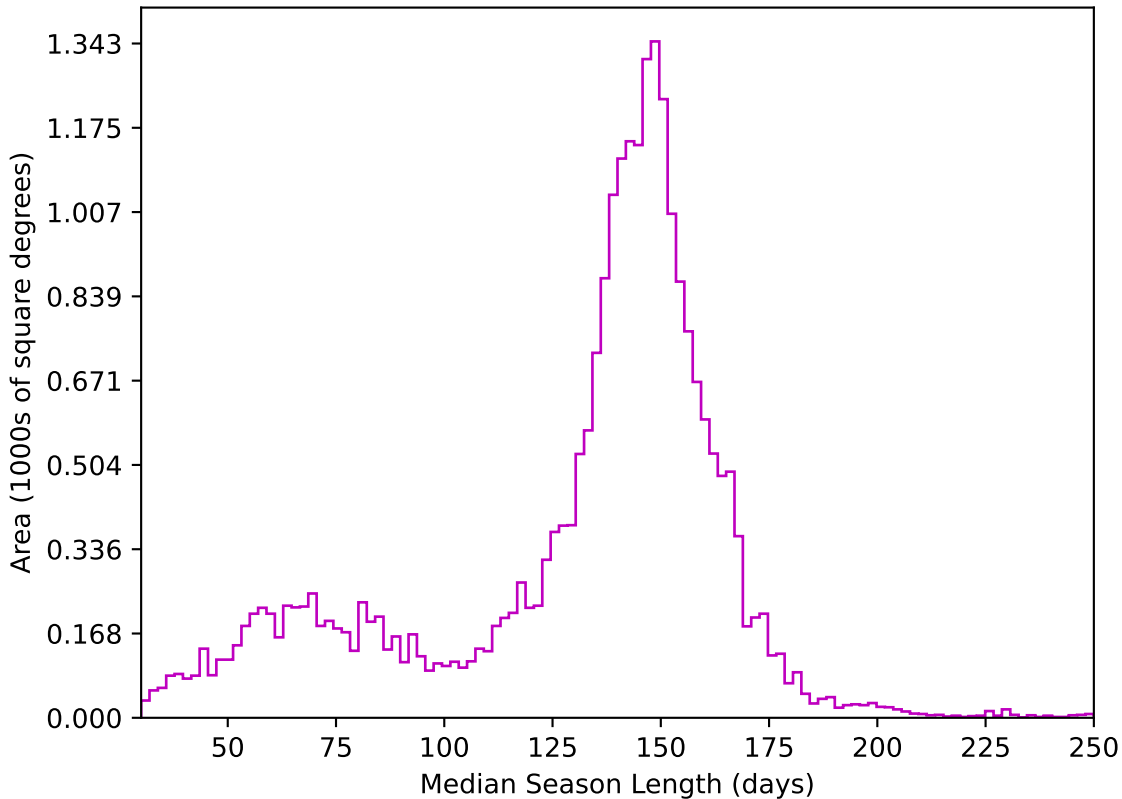
ddf_acor_sf10_lsf15_lsr50_v3.4_10yrs All sky z band: Median Season Length
