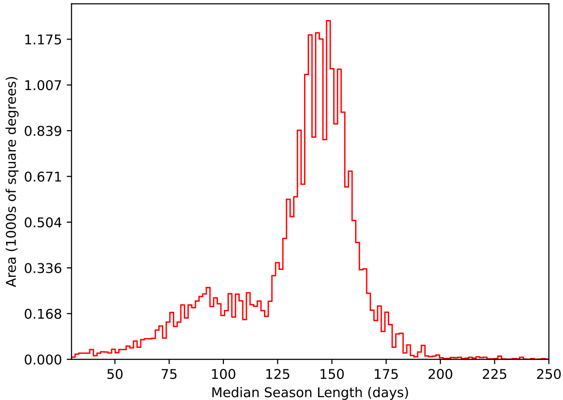
ddf_acor_sf10_lsf15_lsr50_v3.4_10yrs All sky i band: Median Season Length
