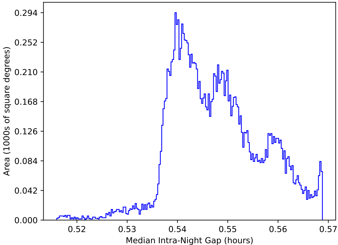
ddf_acor_sf10_ls15_lsr50_v3.4_10yrs WFD: Median Intra-Night Gap
