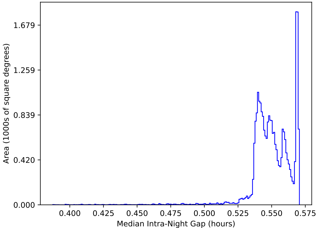
ddf_acor_sf10_lsf15_lsr50_v3.4_10yrs All sky: Median Intra-Night Gap
