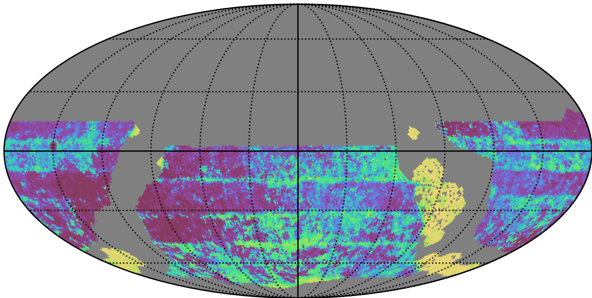
ddf_acor_sf10_lsf15_lsr50_v3.4_10yrs WFD y band: Median Inter-Night Gap
