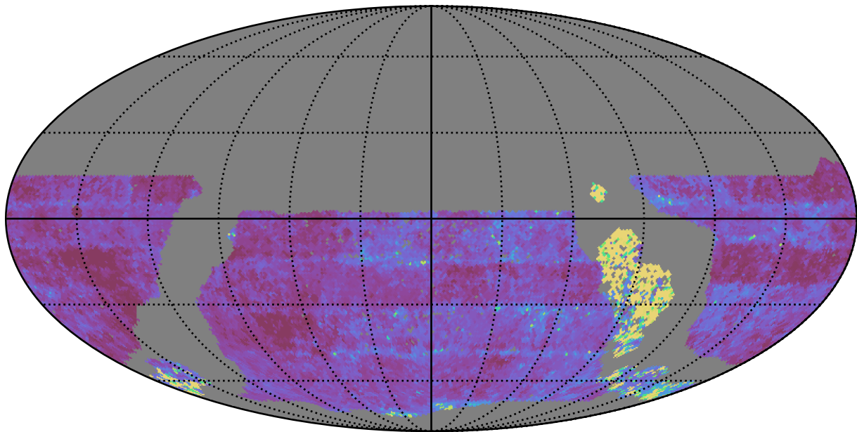
ddf_acor_sf10_lsf15_lsr50_v3.4_10yrs WFD u band: Median Inter-Night Gap
