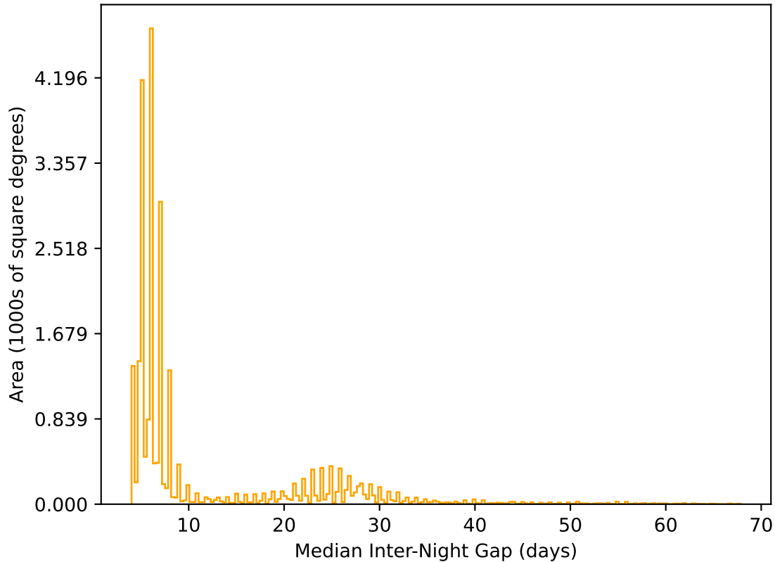
ddf_acor_sf10_lsf15_lsr50_v3.4_10yrs All sky r band: Median Inter-Night Gap
