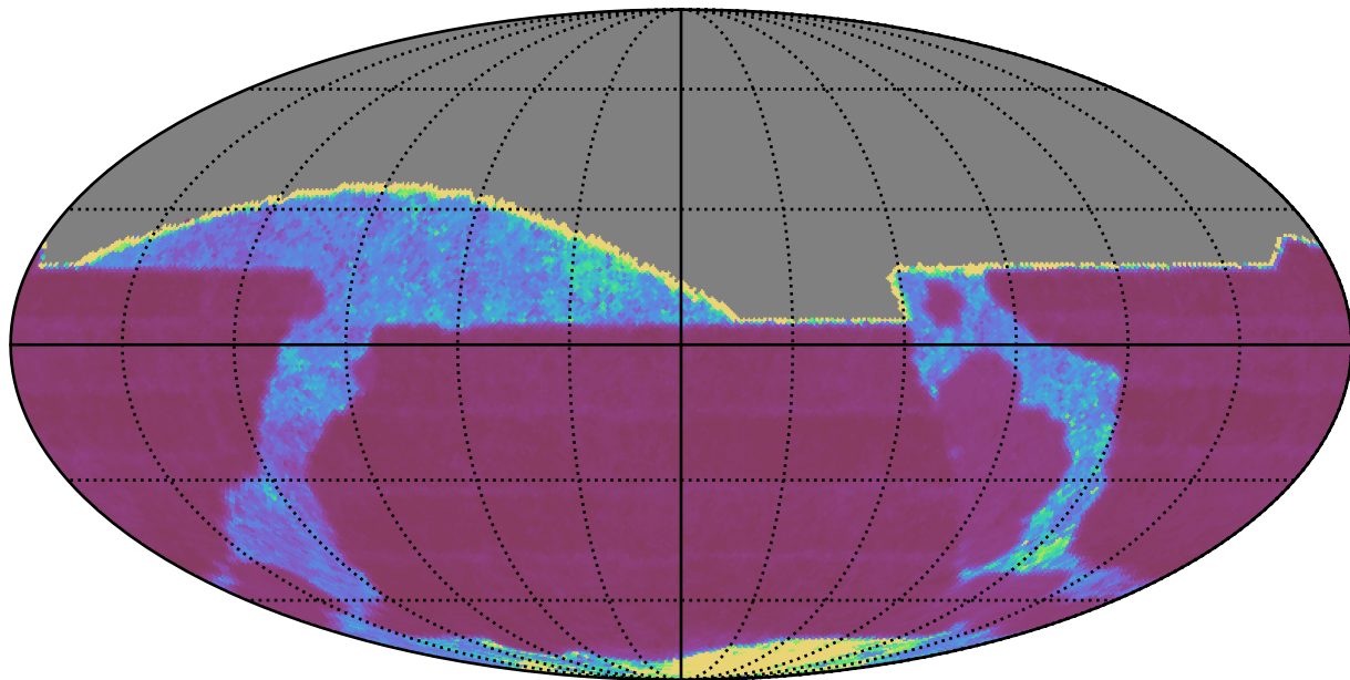
ddf_acor_sf10_lsf15_lsr50_v3.4_10yrs All sky i band: Median Inter-Night Gap
