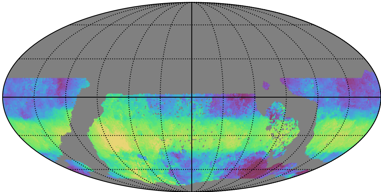
ddf_acor_sf10_lsf15_lsr50_v3.4_10yrs WFD u band: Median HA
