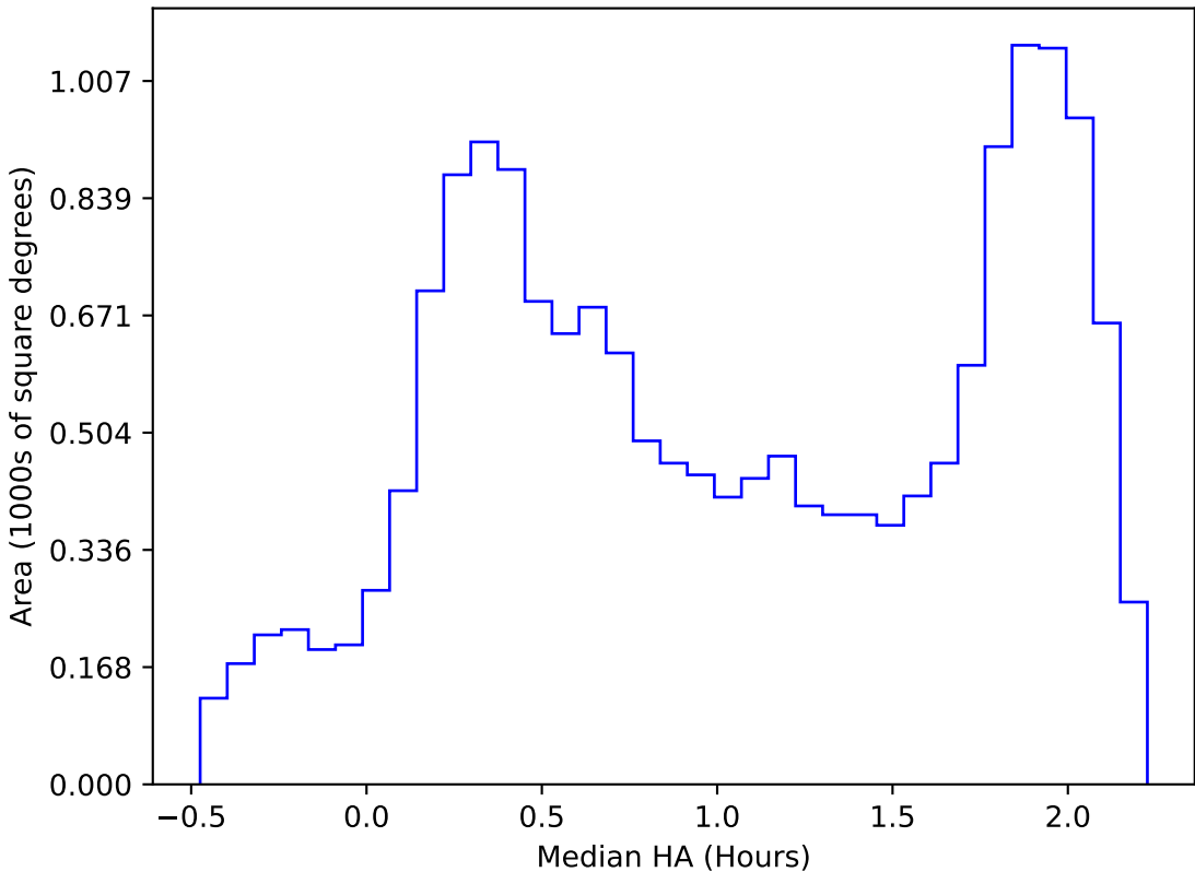
ddf_acor_sf10_lsf15_lsr50_v3.4_10yrs WFD all bands: Median HA
