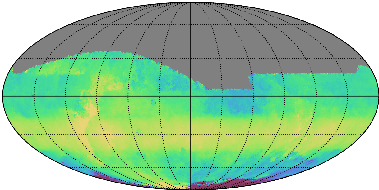
ddf_acor_sf10_lsf15_lsr50_v3.4_10yrs All sky z band: Median HA
