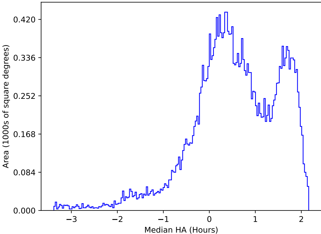
ddf_acor_sf10_lsf15_lsr50_v3.4_10yrs All sky g band: Median HA
