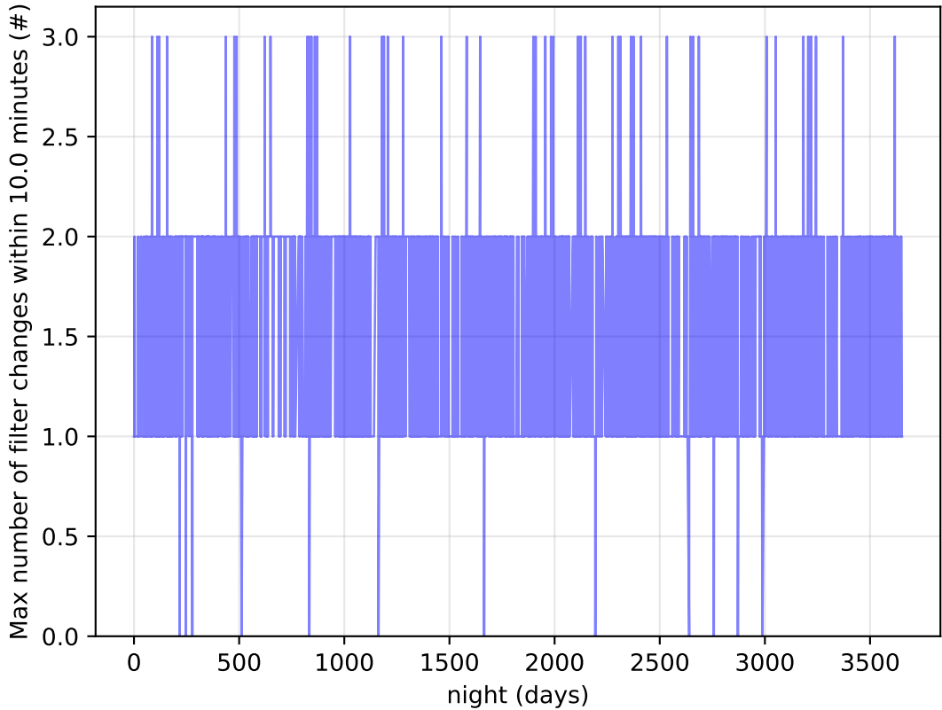
ddf_acor_sf10_Isf15_Isr50_v3.4_10yrs Per Night: Max number of filter changes within 10.0 minutes
