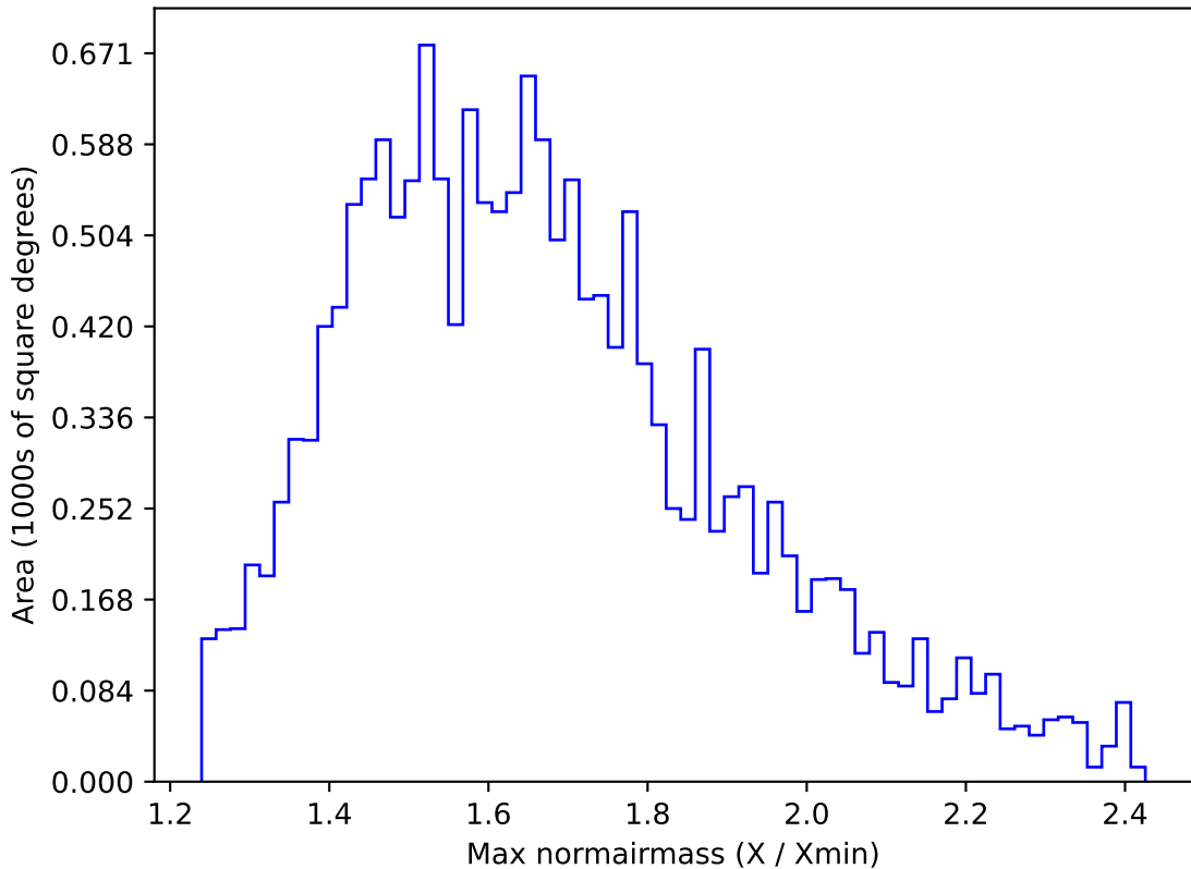
ddf_acor_sf10_lsf15_lsr50_v3.4_10yrs WFD u band: Max normairmass
