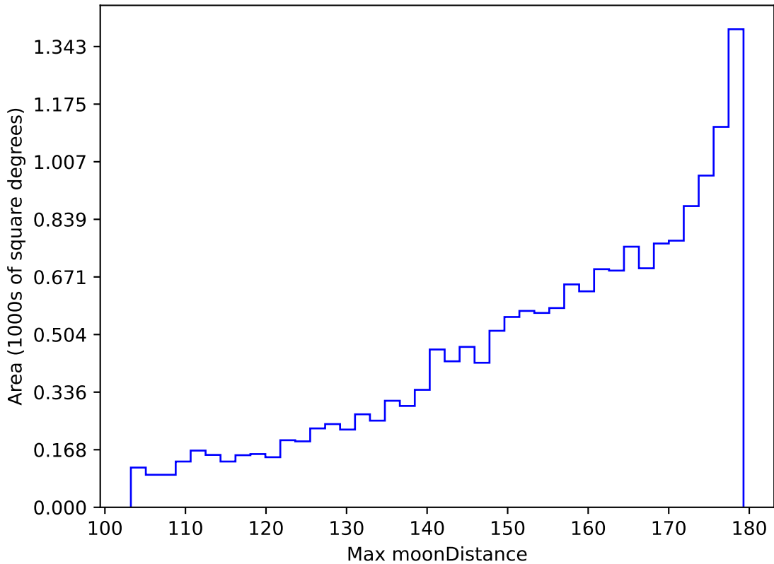
ddf_acor_sf10_lsf15_lsr50_v3.4_10yrs WFD i band: Max moonDistance
