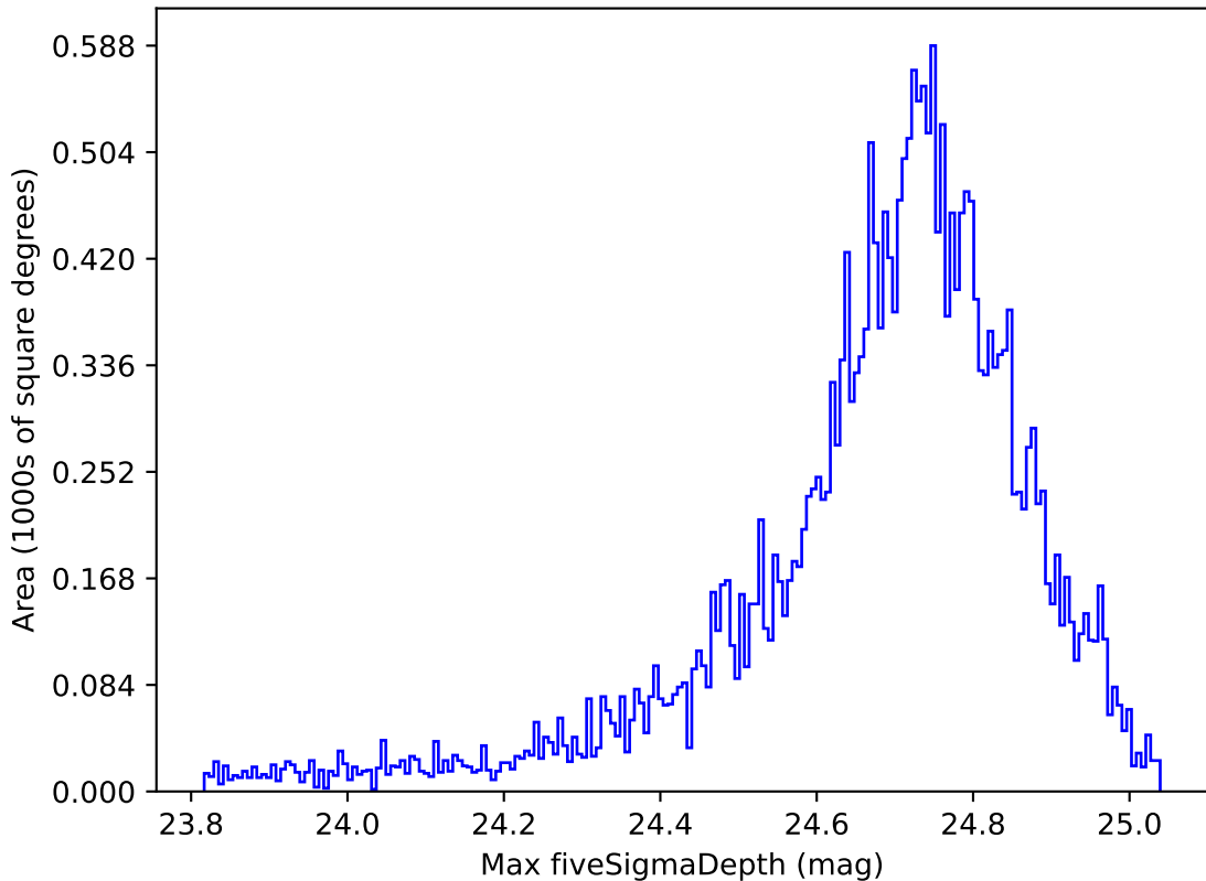
ddf_acor_sf10_lsf15_lsr50_v3.4_10yrs All sky r band: Max fiveSigmaDepth
