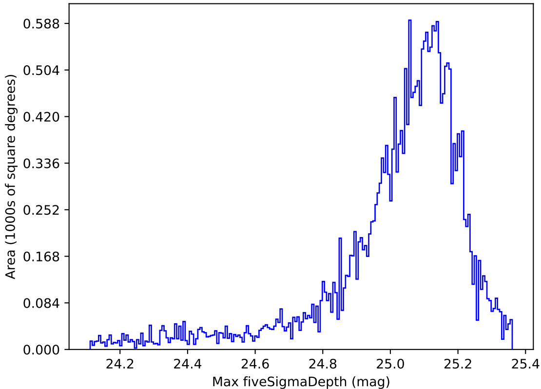
ddf_acor_sf10_ls15_lsr50_v3.4_10yrs All sky g band: Max fiveSigmaDepth
