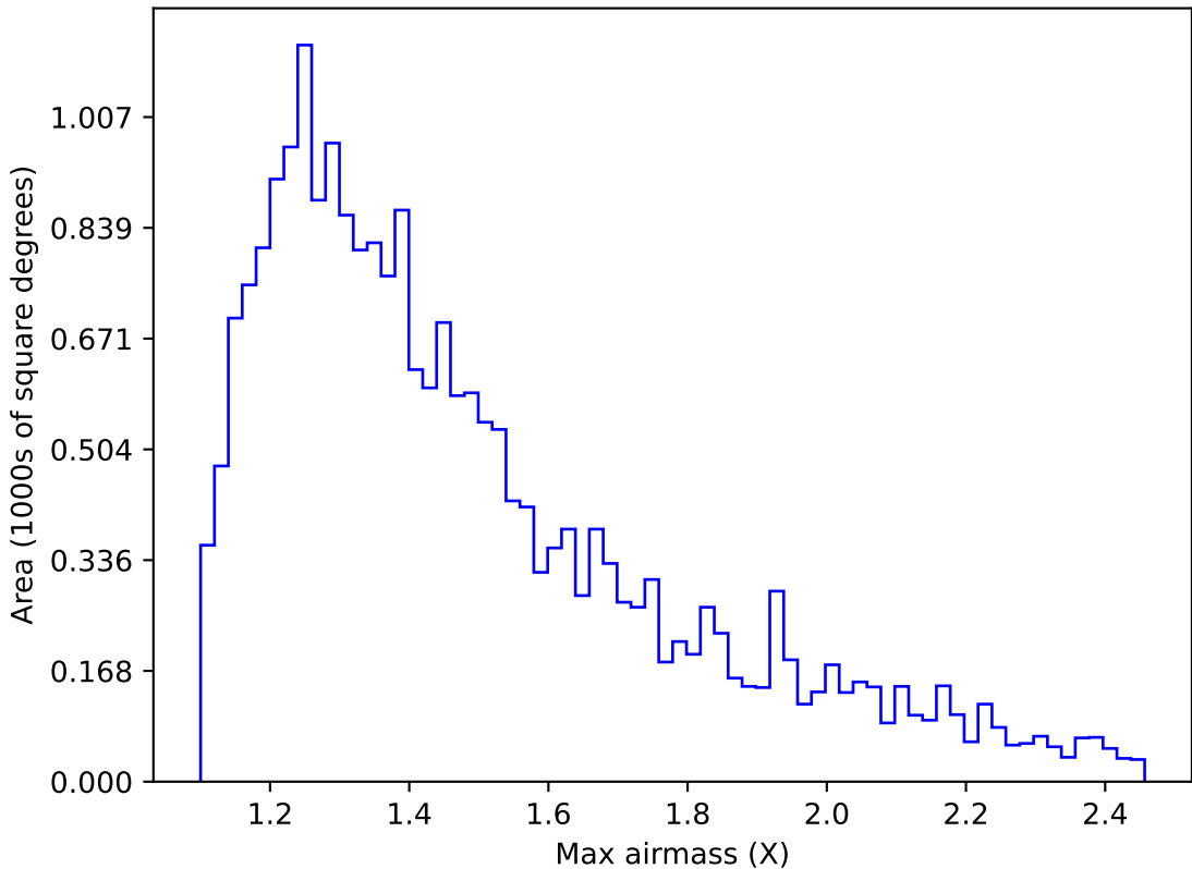
ddf_acor_sf10_lsf15_lsr50_v3.4_10yrs Yr 1 u band: Max airmass
