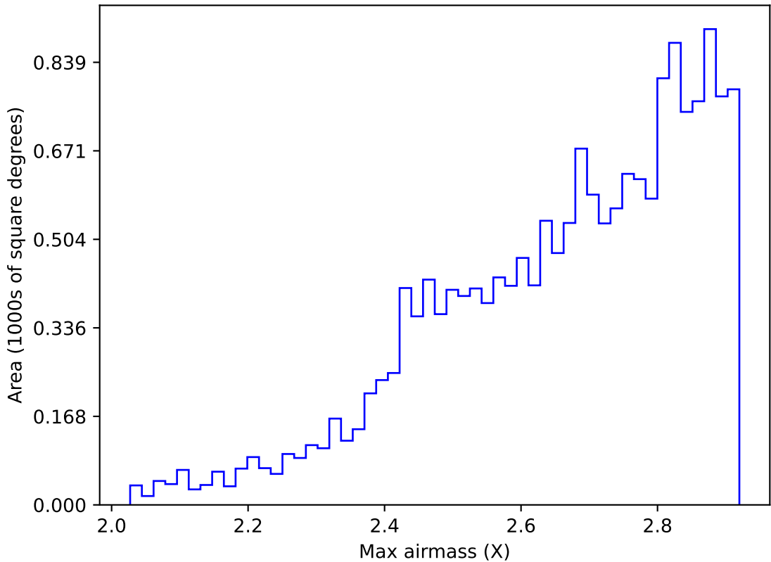
ddf_acor_sf10_lsf15_lsr50_v3.4_10yrs WFD all bands: Max airmass
