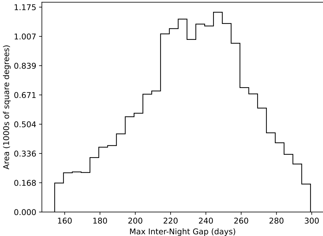
ddf_acor_sf10_lsf15_lsr50_v3.4_10yrs WFD all bands: Max Inter-Night Gap
