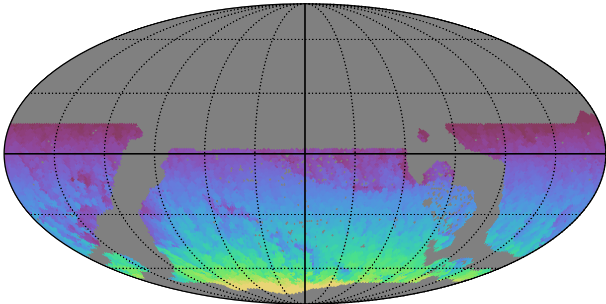
ddf_acor_sf10_lsf15_lsr50_v3.4_10yrs WFD all bands: Max HA
