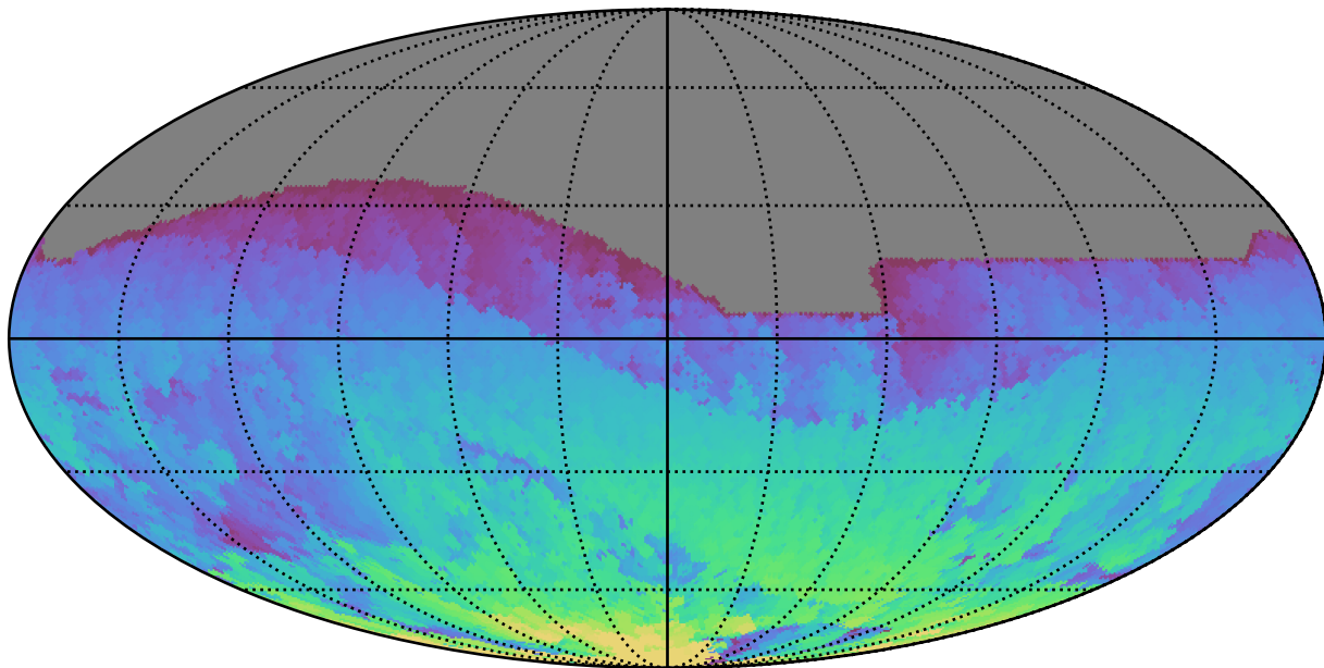
ddf_acor_sf10_lsf15_lsr50_v3.4_10yrs All sky i band: Max HA
