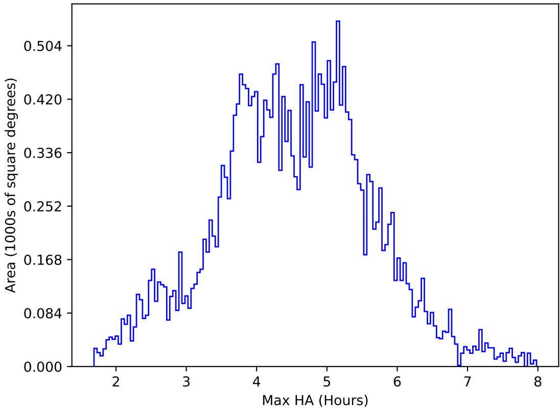
ddf_acor_sf10_lsf15_lsr50_v3.4_10yrs All sky i band: Max HA
