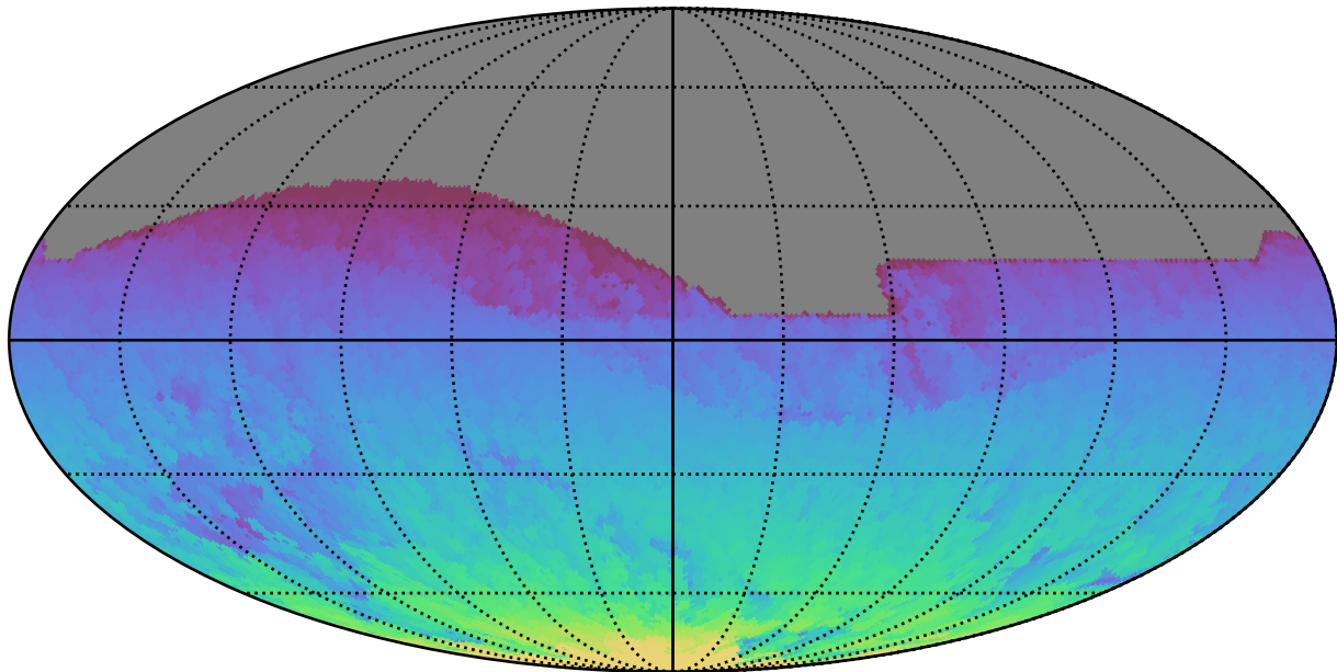
ddf_acor_sf10_lsf15_lsr50_v3.4_10yrs All sky all bands: Max HA
