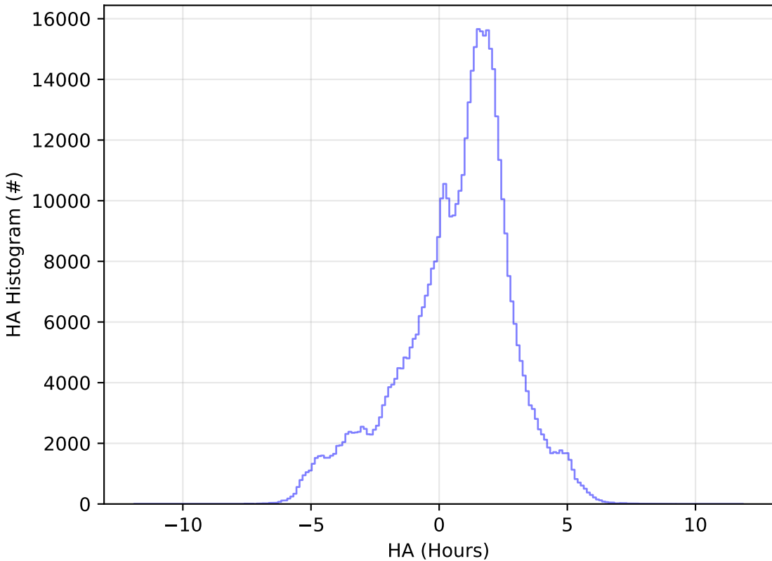
ddf_acor_sf10_lsf15_lsr50_v3.4_10yrs WFD i band: HA Histogram
