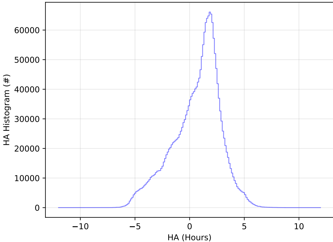
ddf_acor_sf10_lsf15_lsr50_v3.4_10yrs WFD all bands: HA Histogram
