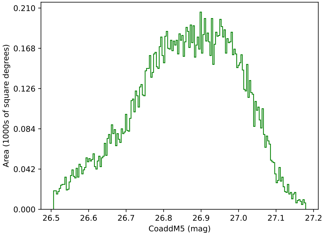
ddf_acor_sf10_lsf15_lsr50_v3.4_10yrs WFD g band: CoaddM5
