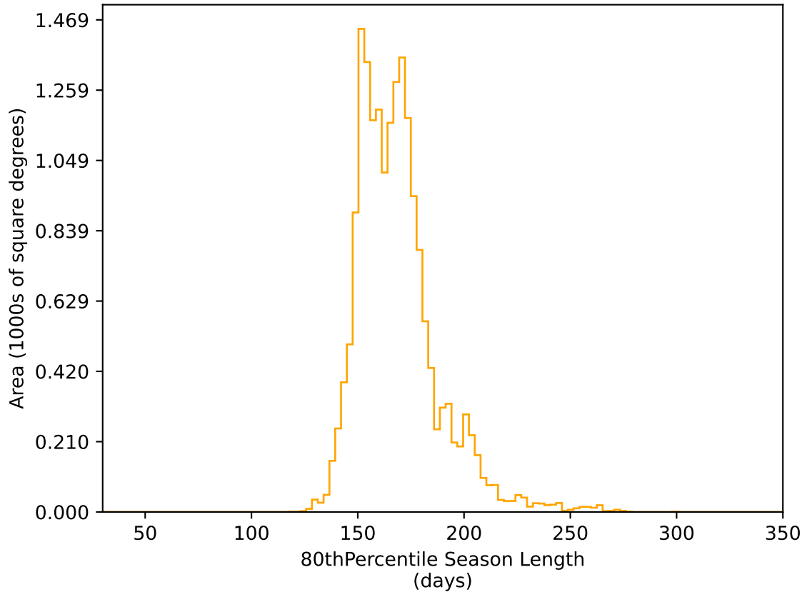
ddf_acor_sf10_lsf15_lsr50_v3.4_10yrs WFD r band: 80thPercentile Season Length
