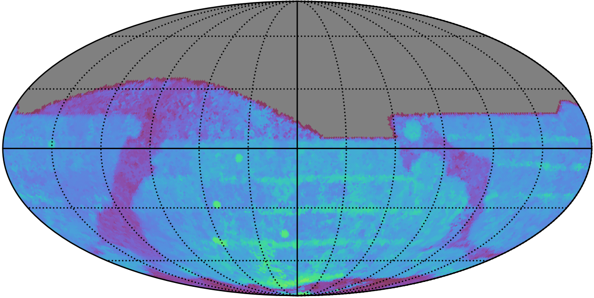
ddf_acor_sf10_lsf15_lsr50_v3.4_10yrs All sky z band: 80thPercentile Season Length
