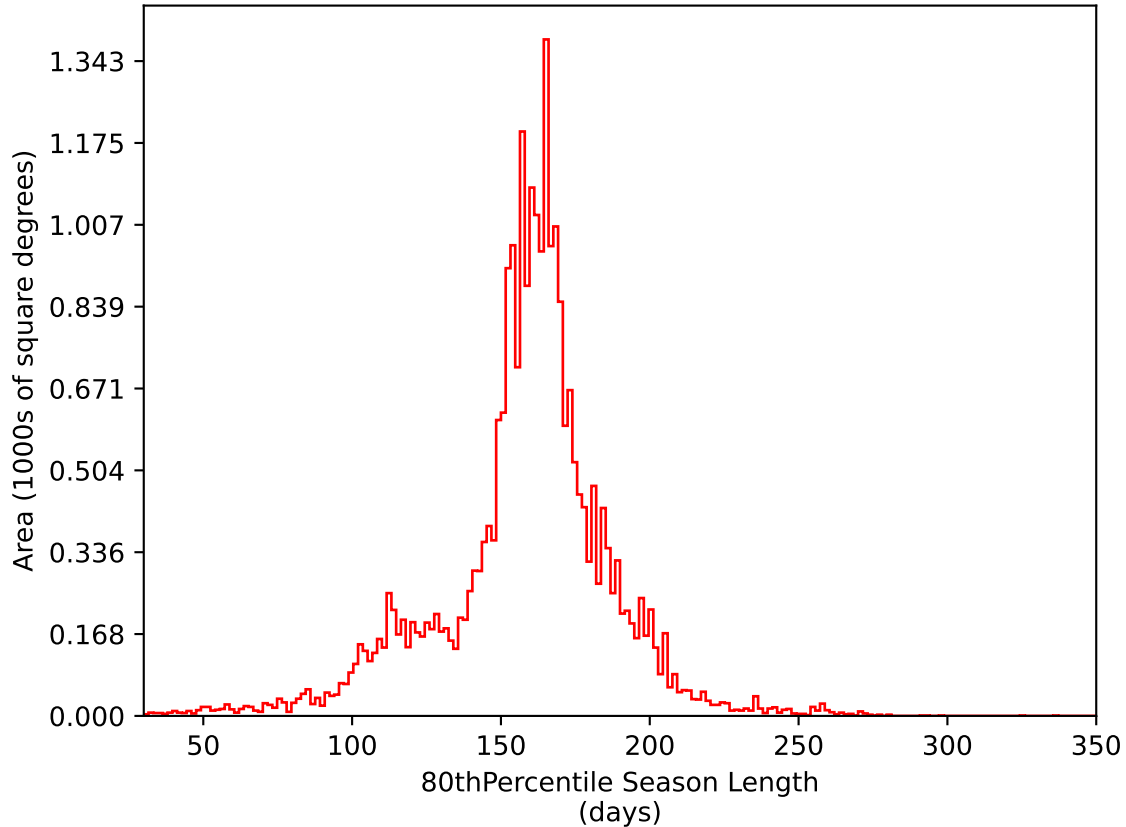
ddf_acor_sf10_lsf15_lsr50_v3.4_10yrs All sky i band: 80thPercentile Season Length
