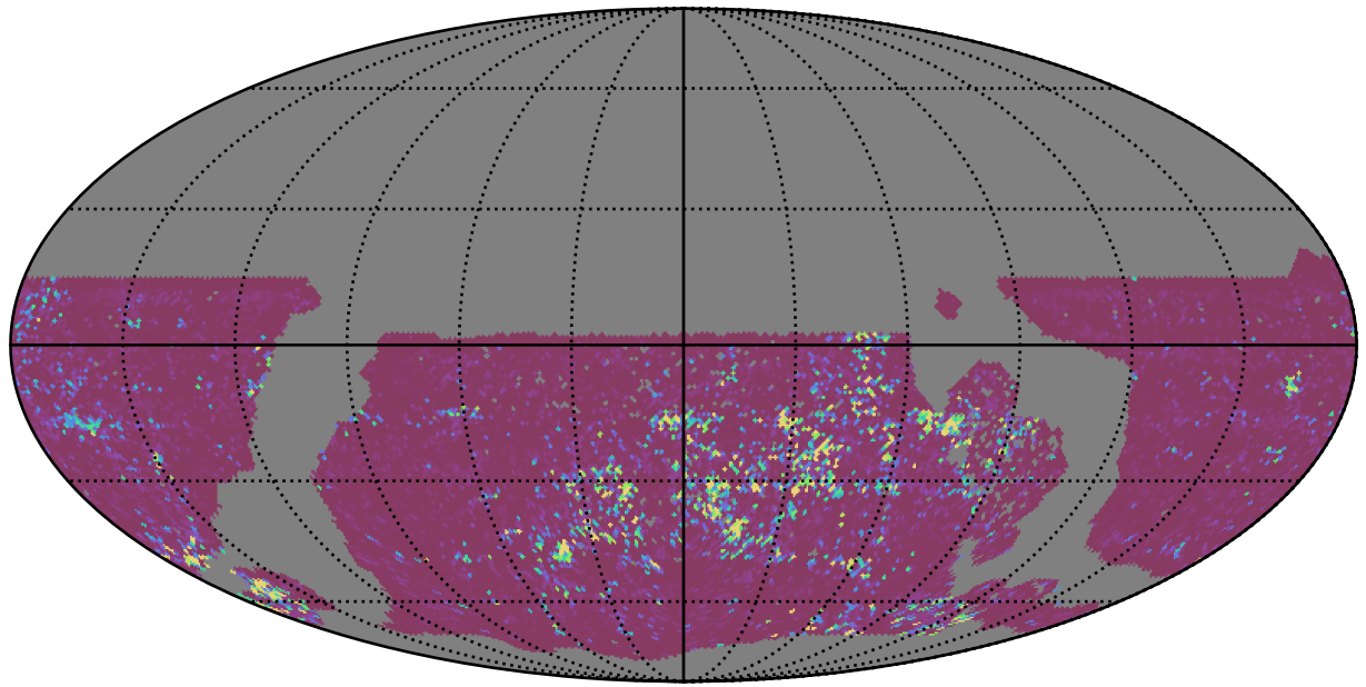
ddf_acor_sf10_lsf15_lsr50_v3.4_10yrs WFD u band: 75th Percentile Intranight Timespan
