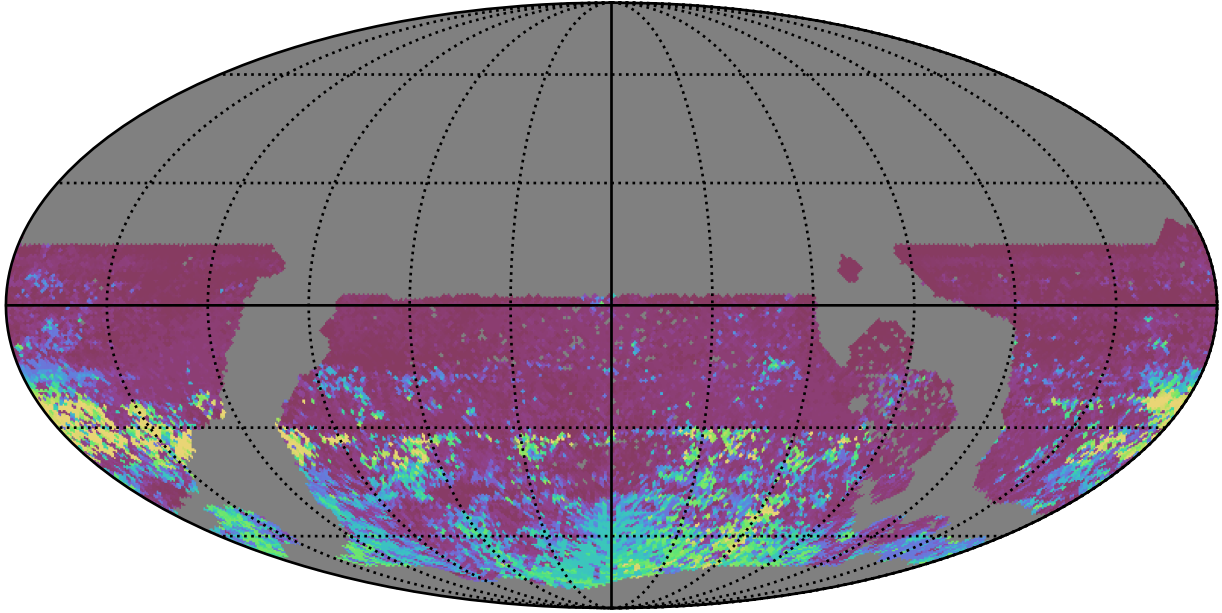
ddf_acor_sf10_lsf15_lsr50_v3.4_10yrs WFD r band: 75th Percentile Intranight Timespan
