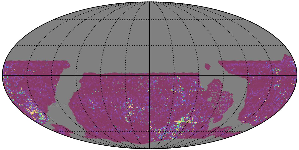
ddf_acor_sf10_lsf15_lsr50_v3.4_10yrs WFD g band: 75th Percentile Intranight Timespan
