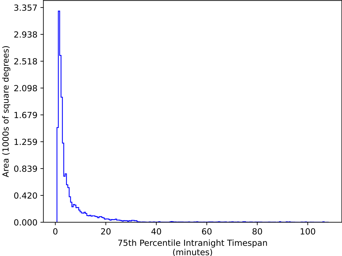
ddf_acor_sf10_lsf15_lsr50_v3.4_10yrs WFD g band: 75th Percentile Intranight Timespan
