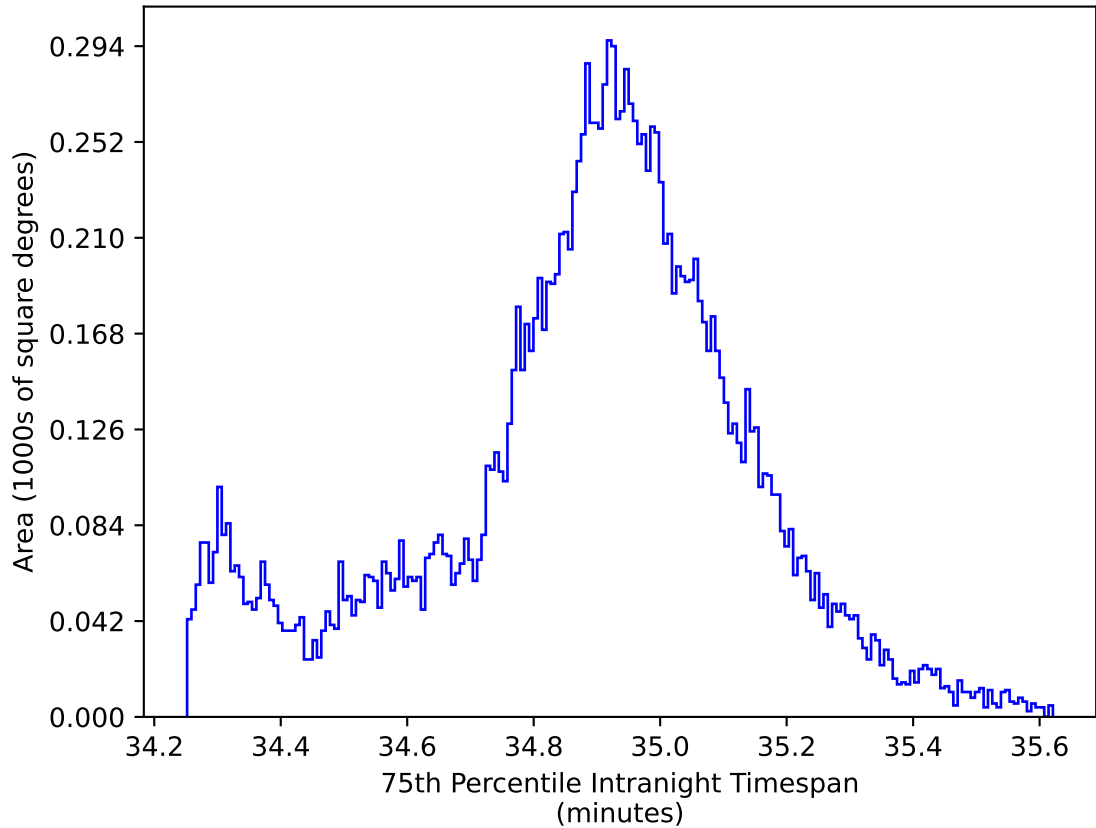
ddf_acor_sf10_lsf15_lsr50_v3.4_10yrs WFD: 75th Percentile Intranight Timespan
