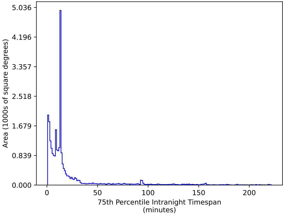
ddf_acor_sf10_ls15_lsr50_v3.4_10yrs All sky z band: 75th Percentile Intranight Timespan
